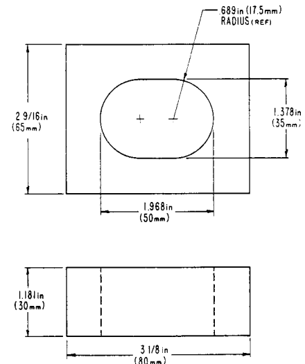
FIG. 15 Rattle Test Fixture
