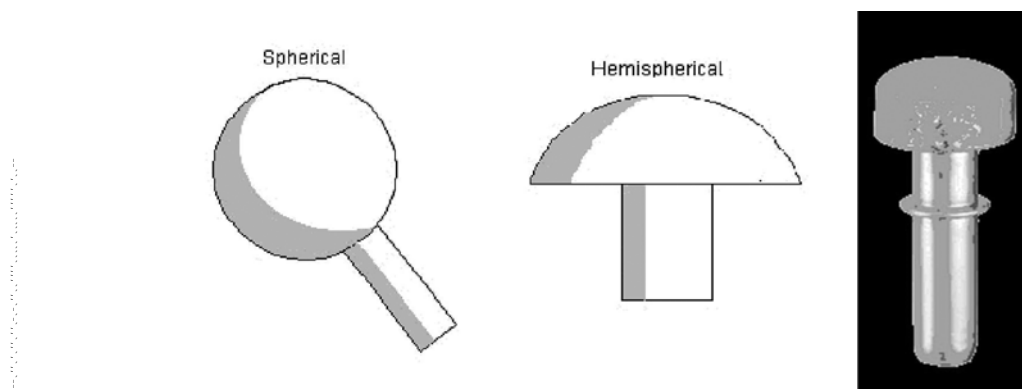
FIG. 17 Examples of Spherical and Hemispherical Ends
