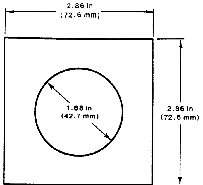
FIG. 15 Rattle Test Fixture
