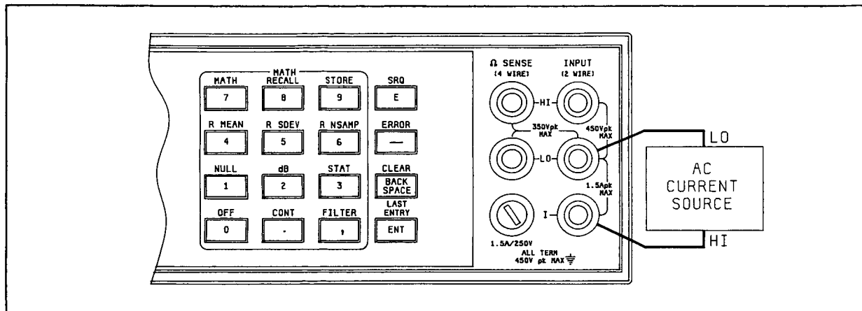
Figure 4-4. ACI Performance Test Connections
