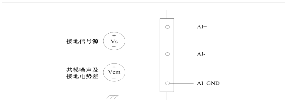
图 4-5-6 接地信号源的差分 (DIFF) 连接
