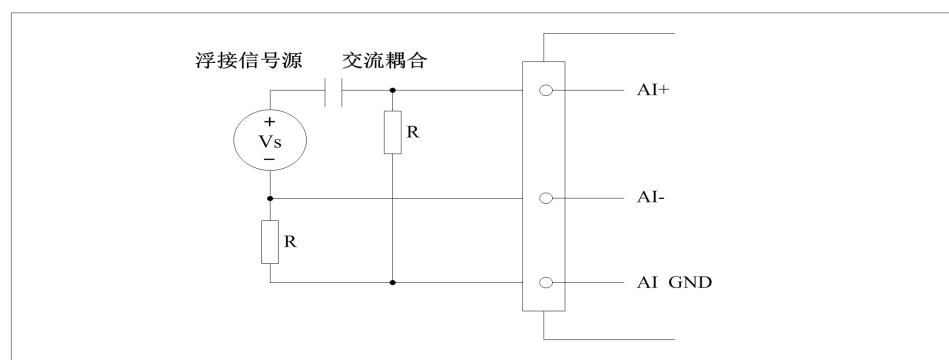
图 4-5-4 浮接信号源差分 (DIFF)连接 ——交流耦合信号源平衡偏置电阻连接
