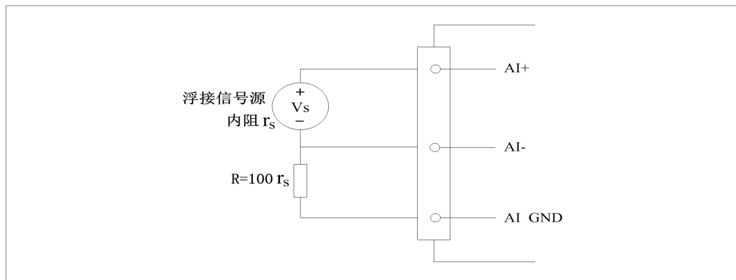
图 4-5-2 浮接信号源差分 (DIFF)连接 -- 单个偏置电阻连接
