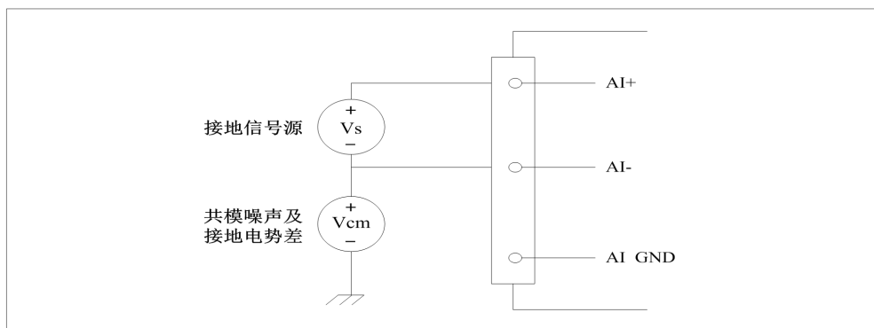
图 4-5-6 接地信号源的差分 (DIFF) 连接
