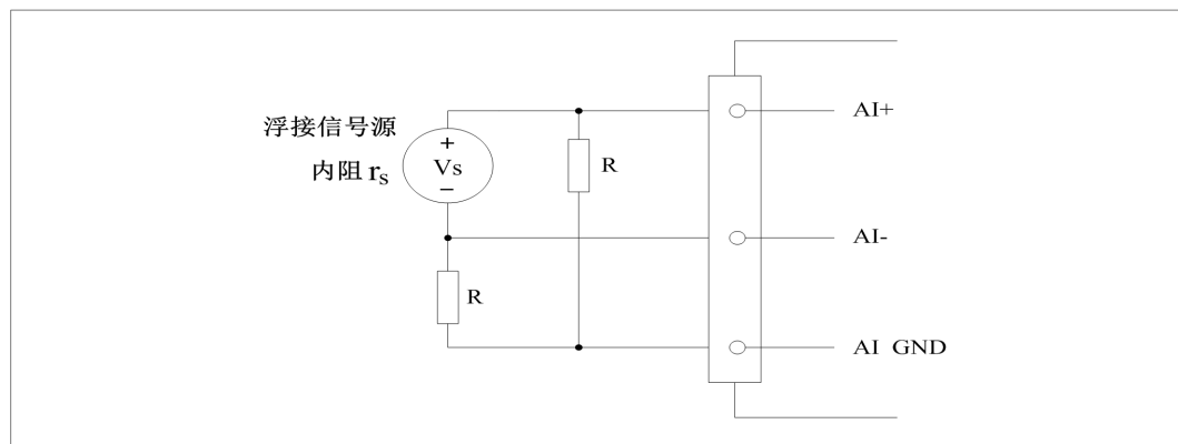
图 4-5-3 浮接信号源差分 (DIFF)连接 -- 平衡偏置电阻连接
