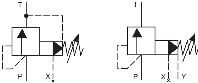
Control oil: internal drainage Control oil: external drainage (Y)
