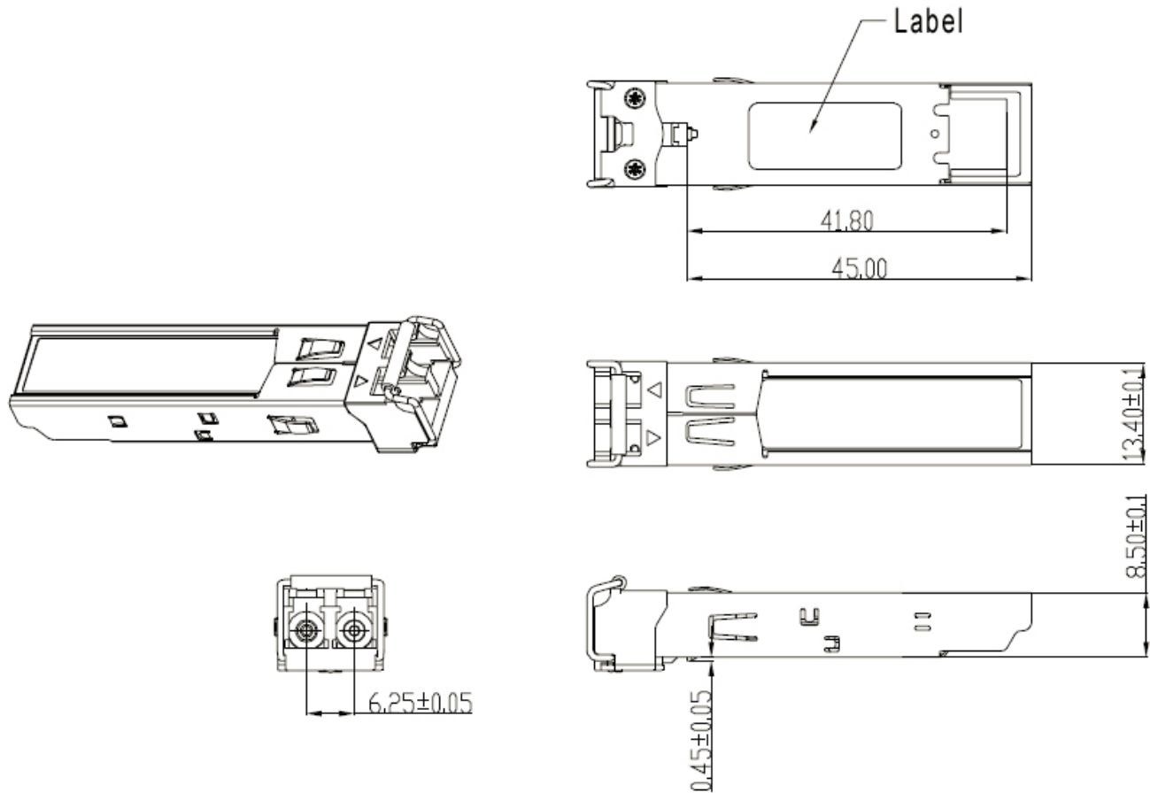
Figure4. Host-Module Interface
