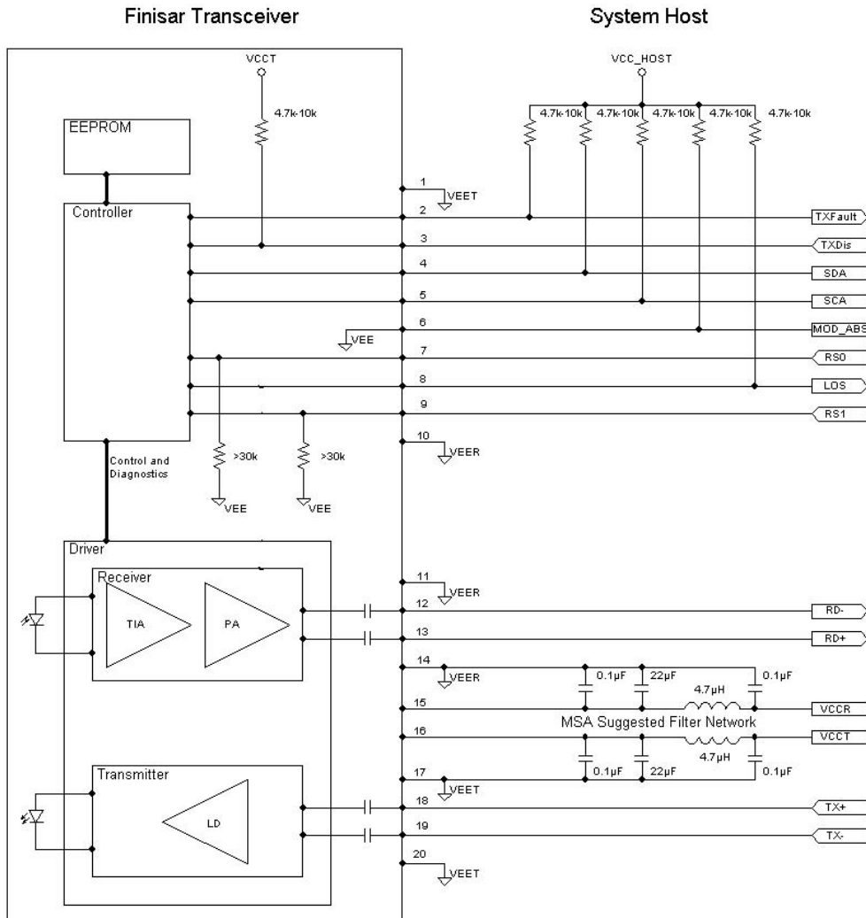
Figure 6-Host-Module Interface
