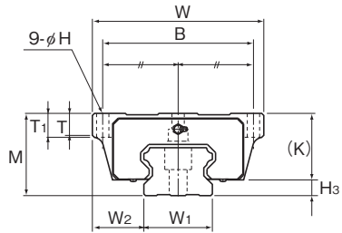
HSR100~150HB型
