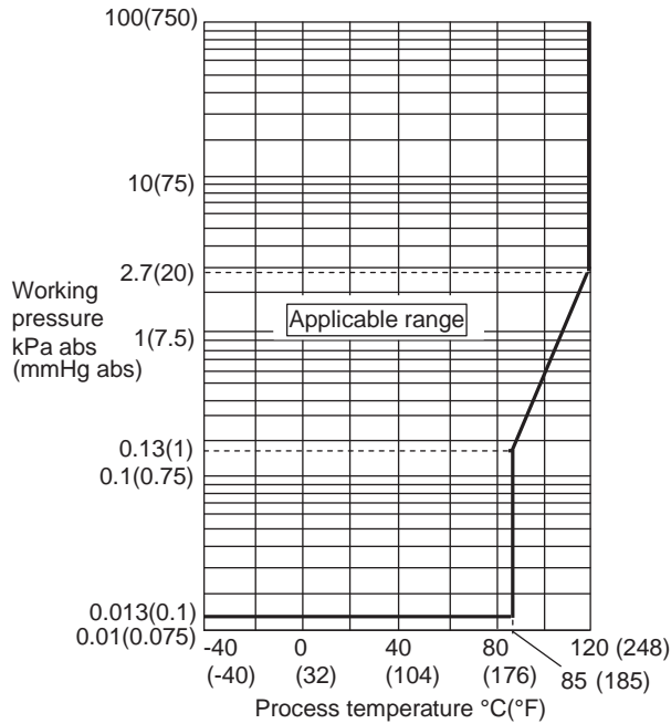
Figure 1-1. Working Pressure and Process Temperature [For EJA510E]
