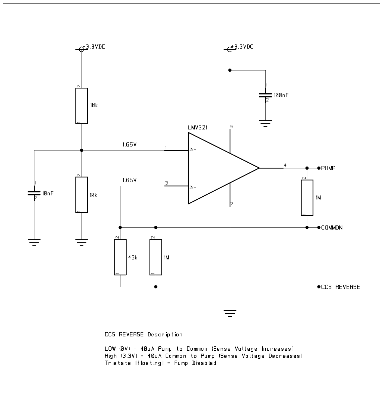
Fig. 5: Microprocessor controlled constant current source
