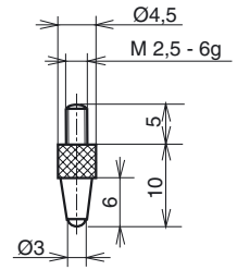
Standard measuring contact
