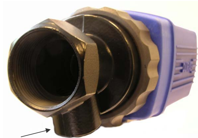
Purge air connection 1/2" screw connection with female thread Commissioning
