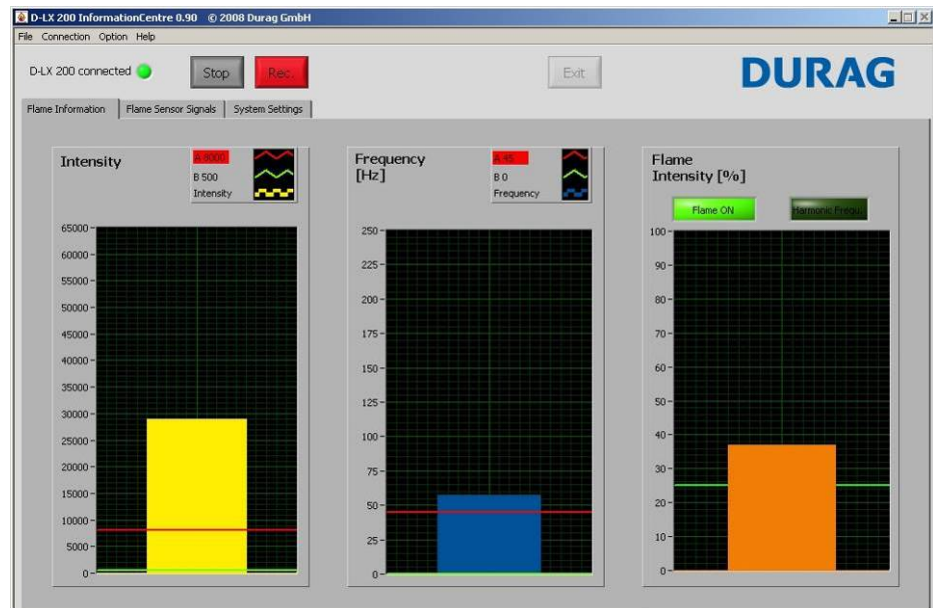
Figure 7.4: Display view Flame Information
