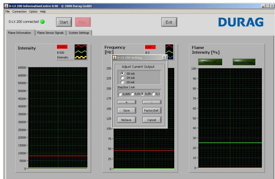
Figure 7.9: "Adjust CurrentOutput" submenu
