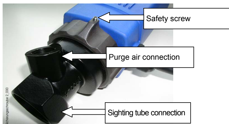
Figure 5.1: Safety screw
