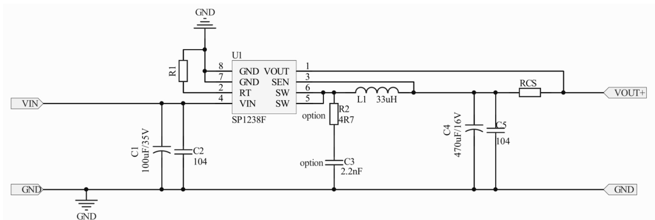
Figure1 Typical Application of SP1238F
