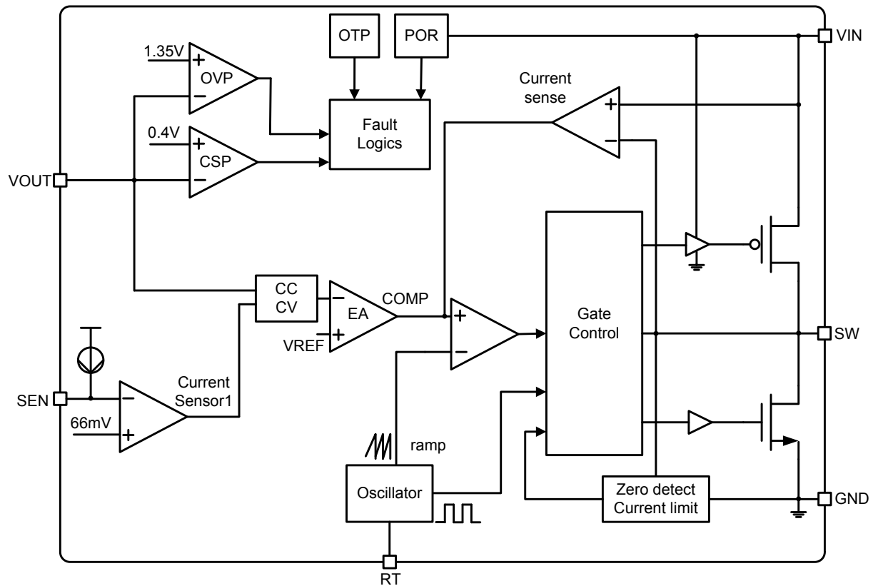
Figure 3 Block diagram of SP1238F
