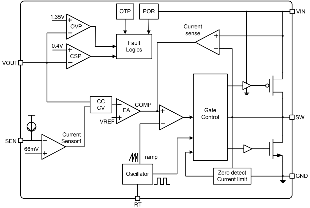
Figure 3 Block diagram of SP1237F
