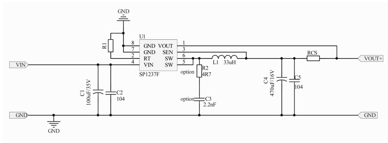
Figure1 Typical Application of SP1237F
