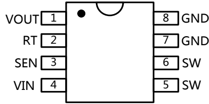
Figure 2 Pin Configuration
