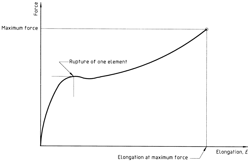
Figure 3 — Rupture of one element of a coated fabric
