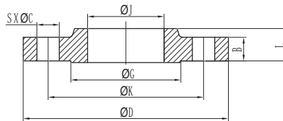
Slip-on Flange
