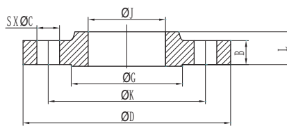
Slip-on Flange
