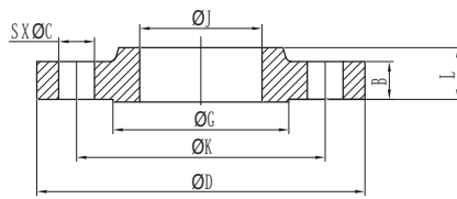
Slip-on Flange
