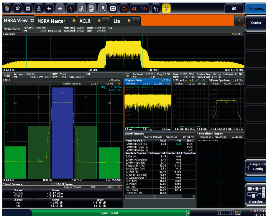
Multiview display of two LTE signals measured on the same I/Q data for interference analysis.
