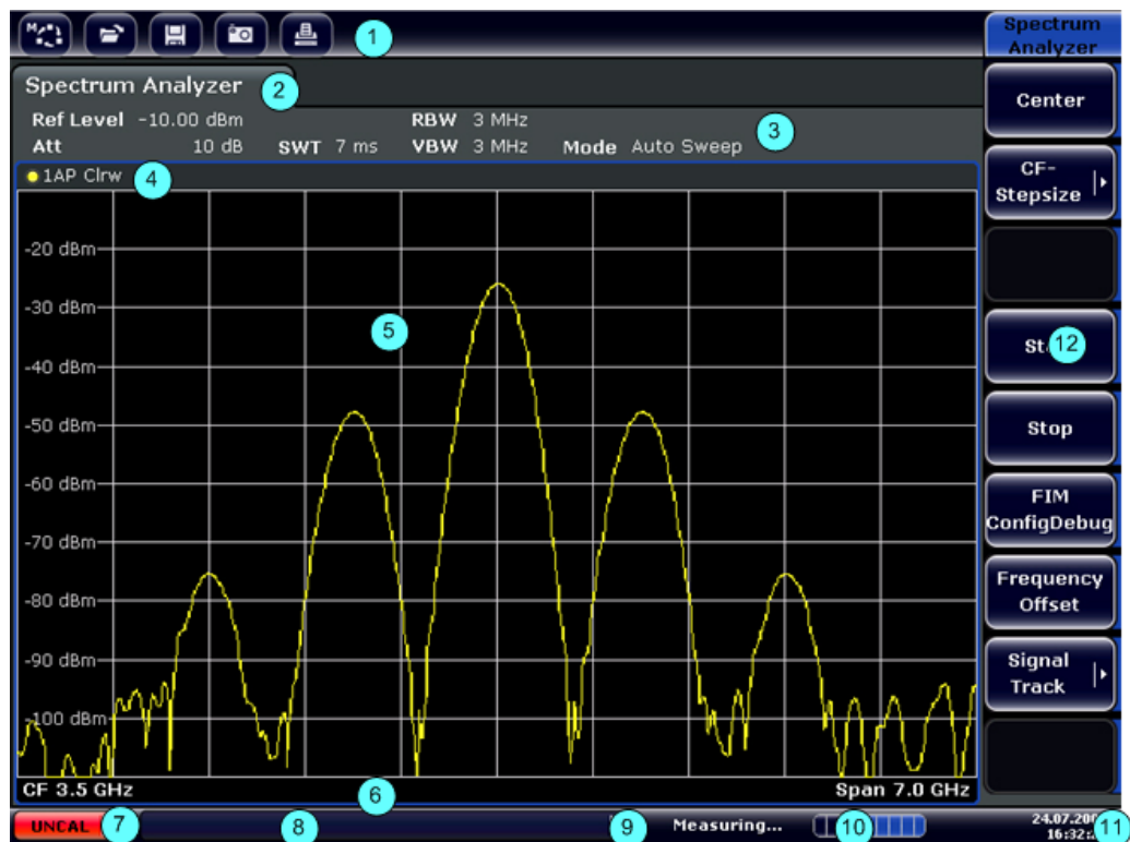
Figure 3-2: Touchscreen elements
