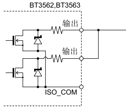
Wired OR
