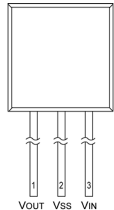
TO-92 (SIDE VIEW)
