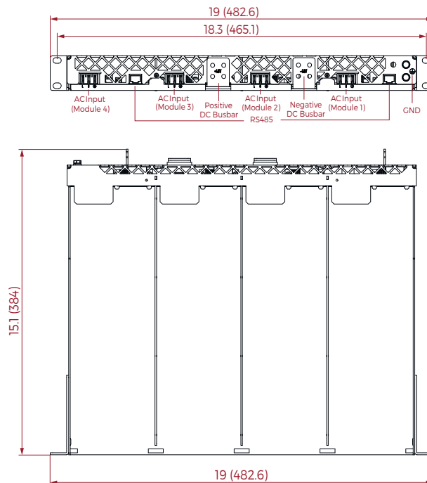
XG1948C - Top and rear view with position and description of connectors
