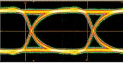
Verify and debug your HDMI designs
