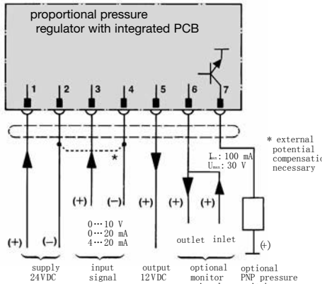
connection diagram
