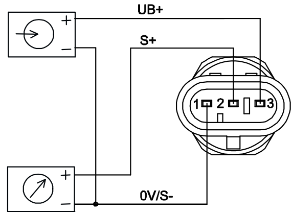
AMP Superseal
