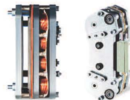
INTORQ.BFK466
