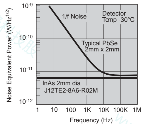
Figure 13-5 Example of NEP vs. Frequency
