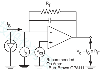
Figure 3 Basic Operating Circuit for InSb
