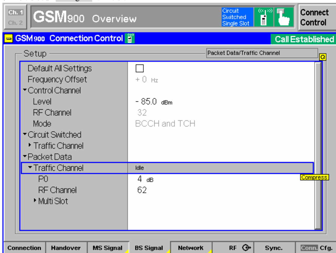
图 2—10 GSM900 Connetion Control_BS Signal_Press Twice
