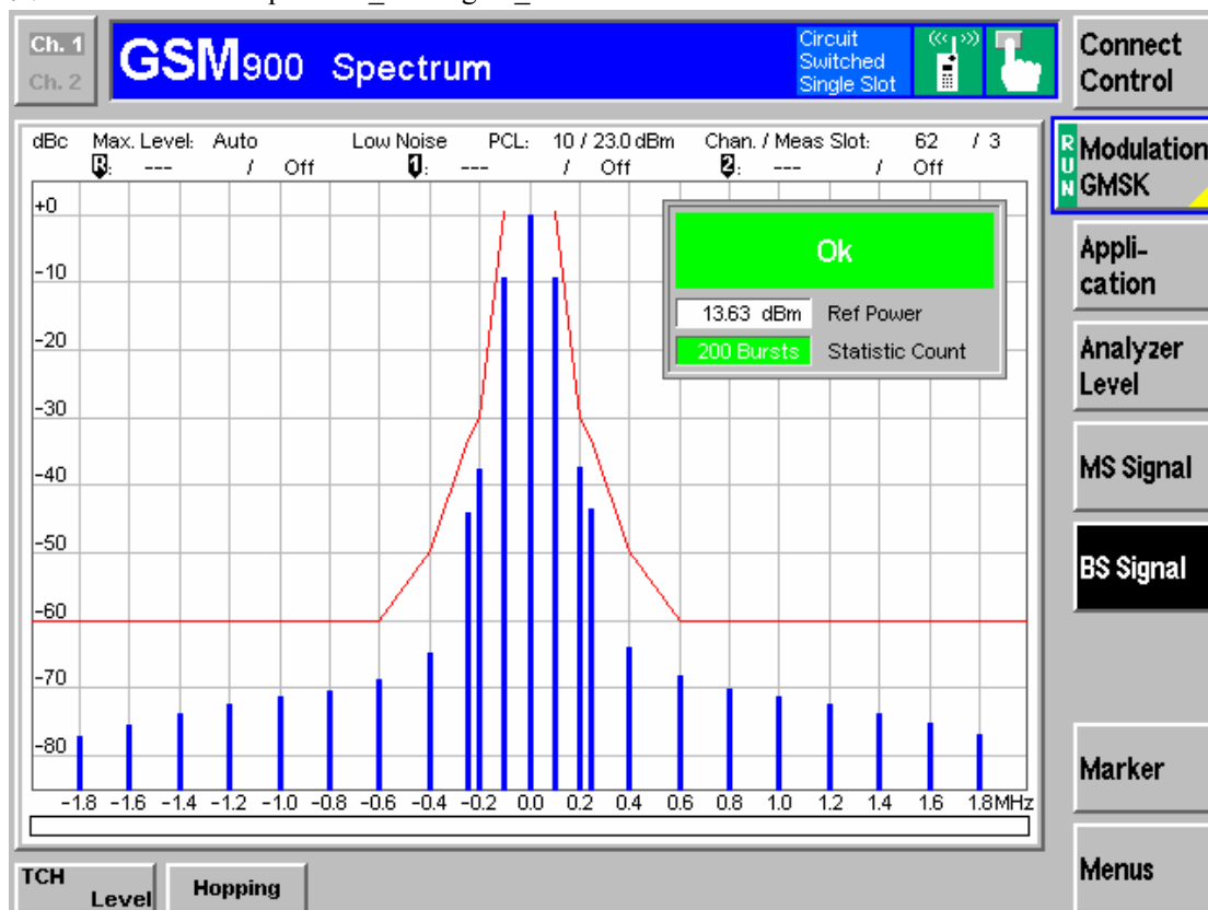
图 2—47 GSM900 Spectrum_BS Signal_Modulation GMSK
