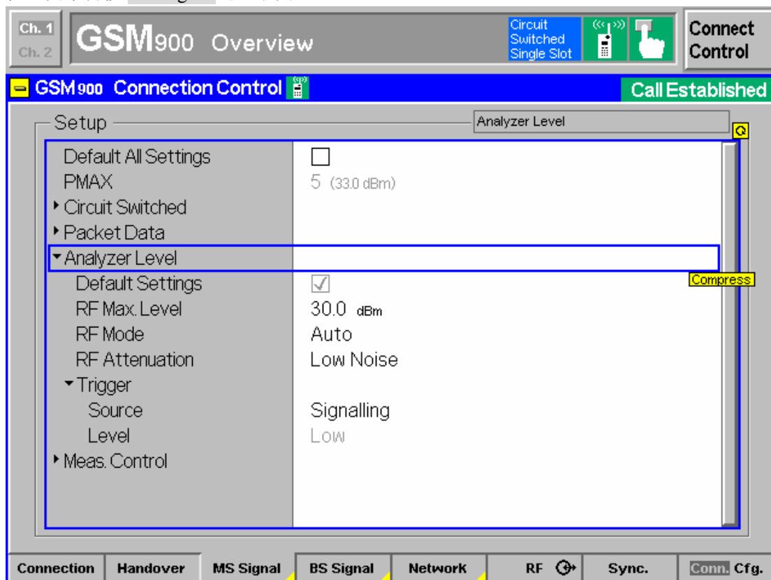
图 2_8 GSM900 Connetion Control_MS Signal_Press Twice
