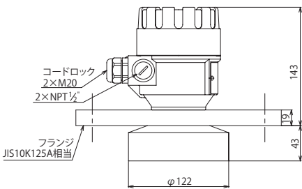
S□□-44P-□ / PP,PVDF
