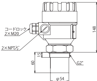
S□□-480-□ / PP,PVDF,PTFE
