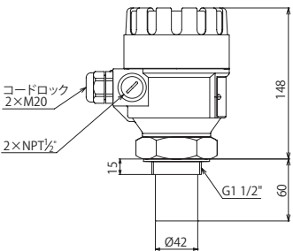
S□□-490-□ / PP,PVDF,PTFE
