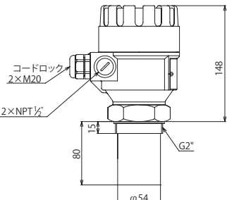
S□□-470-□ / PP,PVDF,PTFE
