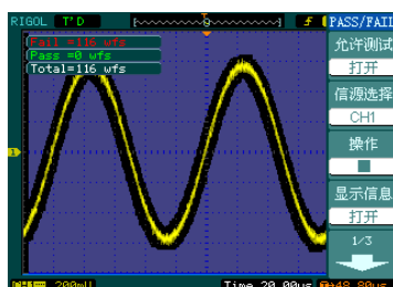
Pass/Fail 检测
