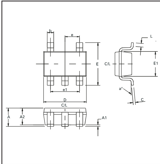
SOT23-5 PACKAGE OUTLINE
