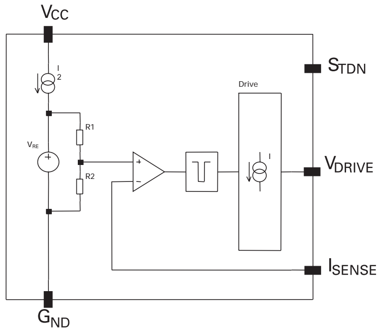
310 Block Diagram
