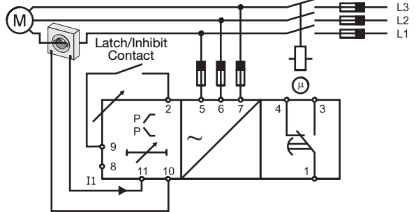
PWB02 - Standard CT
