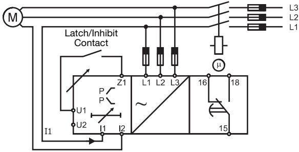
DWB02 - Direct connection
