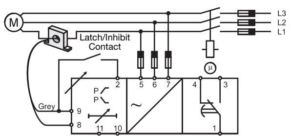
PWB02 - MI CT
