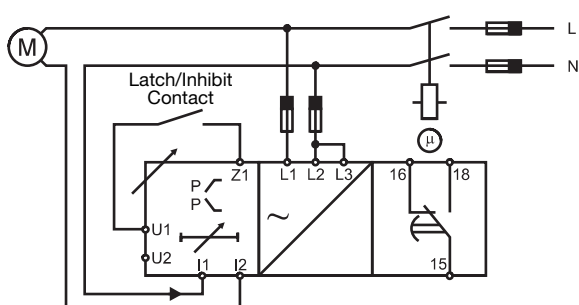
DWB02CM2310A - Direct connection - 1-Phase Load
