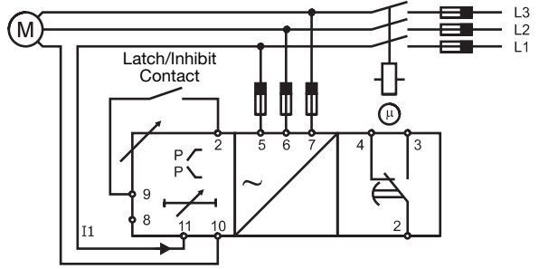
PWB02 - Direct connection
