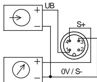
Circular plug-in connector M12x1
