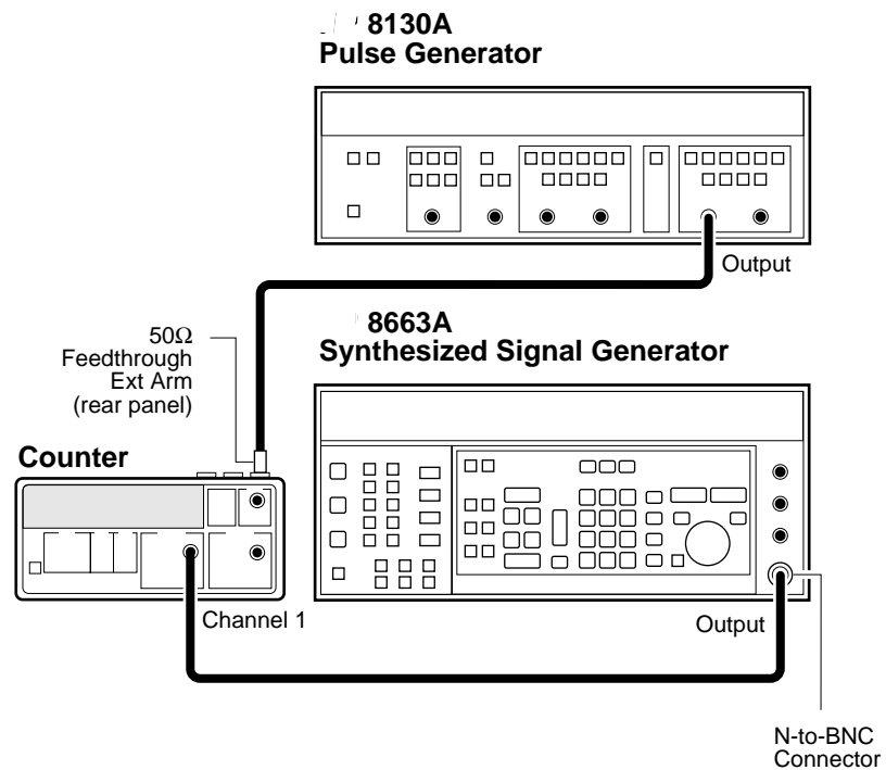
Figure 1-3. External Arm Test Setup (Agilent 53131A/132A Only)
