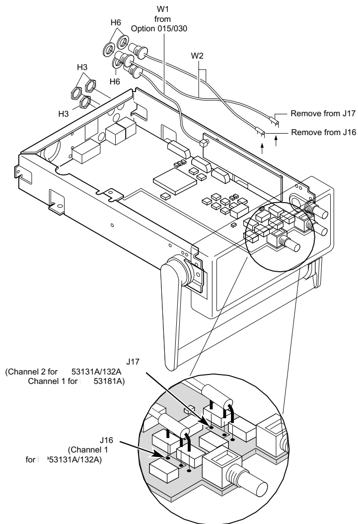
Figure 3-13. Rear Terminals (Option 060) Removal
