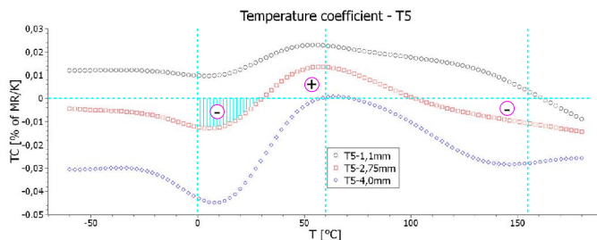
example: zero TC at 0 °C, 60 °C and 155 °C
