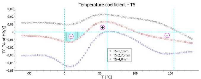
example: zero TC at 0 °C, 60 °C and 155 °C
