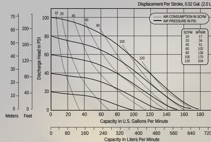
2" (50.8mm) E2 Non-Metallic Bolted
