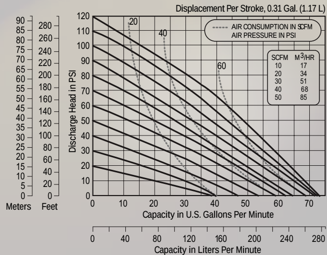
1 1/2" (38mm) E4 Non-Metallic Bolted
