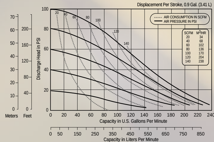
3" (76.2mm) E3 Non-Metallic Bolted
