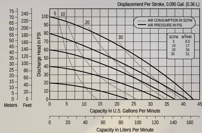
1" (25.4mm) E1 Non-Metallic Bolted
