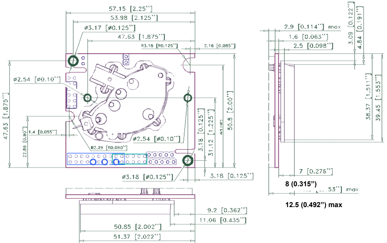
Figure 3. CO 2 Engine® K30 STA mechanical drawing
