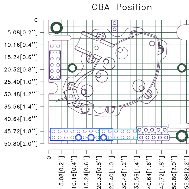
Figure 3. CO 2 Engine ® K30 OBA position.
