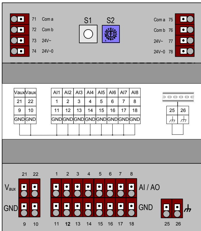
Fig. 9. Excel 800 Analog Input Modules (top view)
