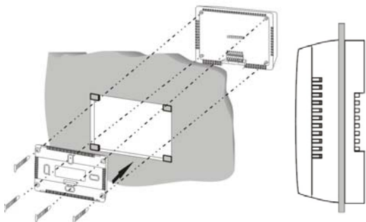
Fig. 5—Panel Front Door Mounting
