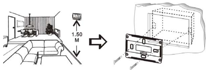
Figure 3—Wall Mounting with Screws
