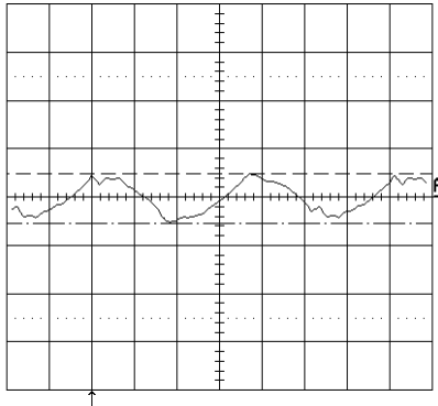
Output voltage ripple (50mV/div.) at T_{Pcb}=+25\text{ }^{\circ}\text{C} , V_{in}=53\text{ V} , I_o=20\text{ A} resistive load. Band width=4MHz. Time scale: 1μs / div.
