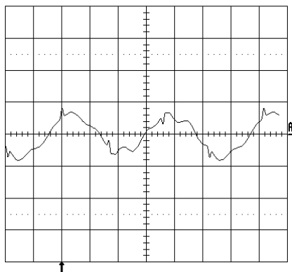
Output voltage ripple (50mV/div.) at T_{Pcb}=+25\text{ }^{\circ}\text{C} , V_{in}=53\text{ V} , I_o=25\text{ A} resistive load. Band width=4MHz. Time scale: 1\mu\text{s} / \text{div} .
