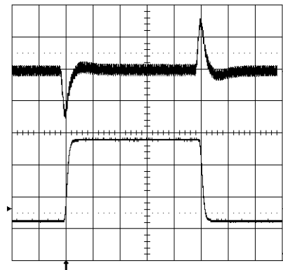
Output voltage response to load current step-change (6.25-18.75-6.25 A) at T_{Pcb}=+25\text{ }^{\circ}\text{C} , V_{in}=53\text{ V} . Top trace: output voltage (200mV/div.). Bottom trace: load current (5 A/div.) Time scale: 0.1\text{ ms/div} .
