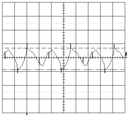
Output voltage ripple (50mV/div.) at T_{Pcb}=+25\text{ }^{\circ}\text{C} , V_{in}=53\text{ V} , I_o=30\text{ A} resistive load. Band width=4MHz. Time scale: 2\mu\text{s} / \text{div} .
