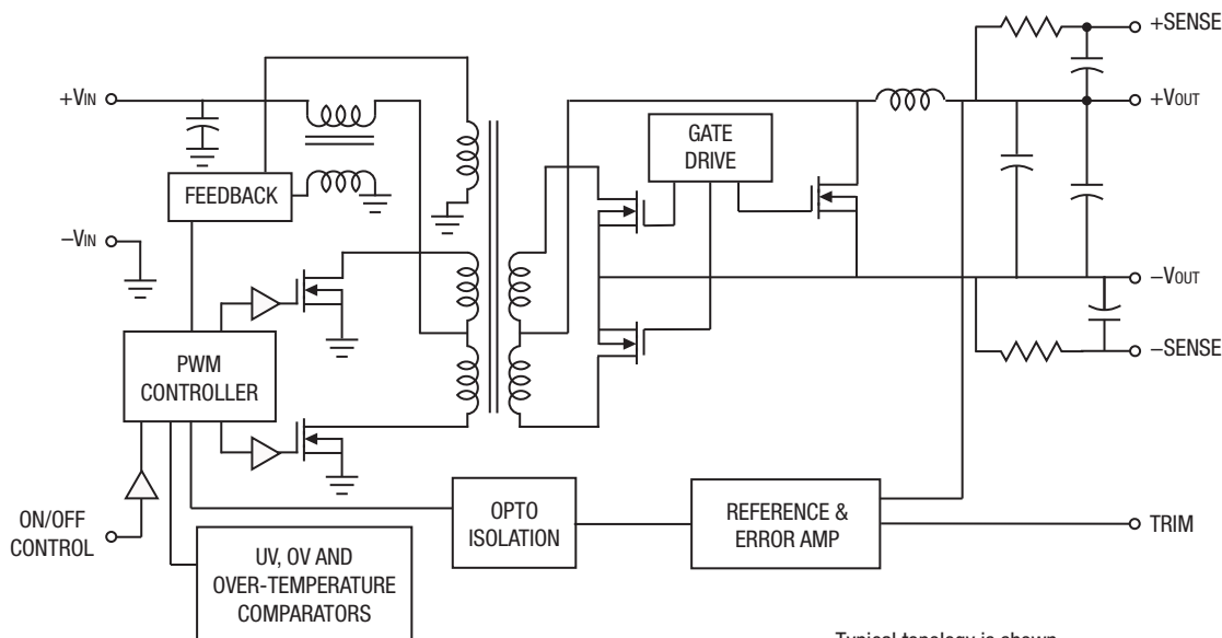
ULE-3.3/20-D48N
