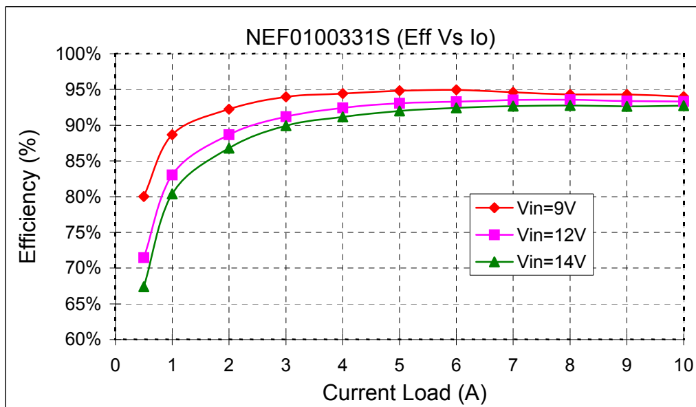
Figure 16. Efficiency Curves for Vout=3.3V (25C)
