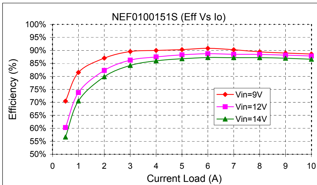
Figure 12. Efficiency Curves for Vout=1.5V (25C)
