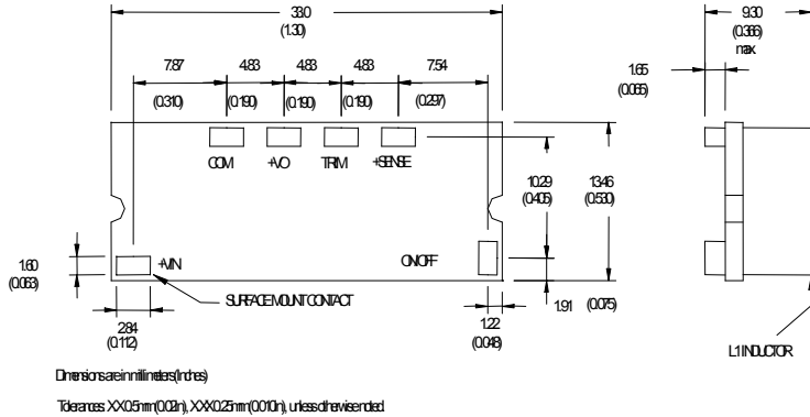
BOTTOM VIEW OF BOARD
