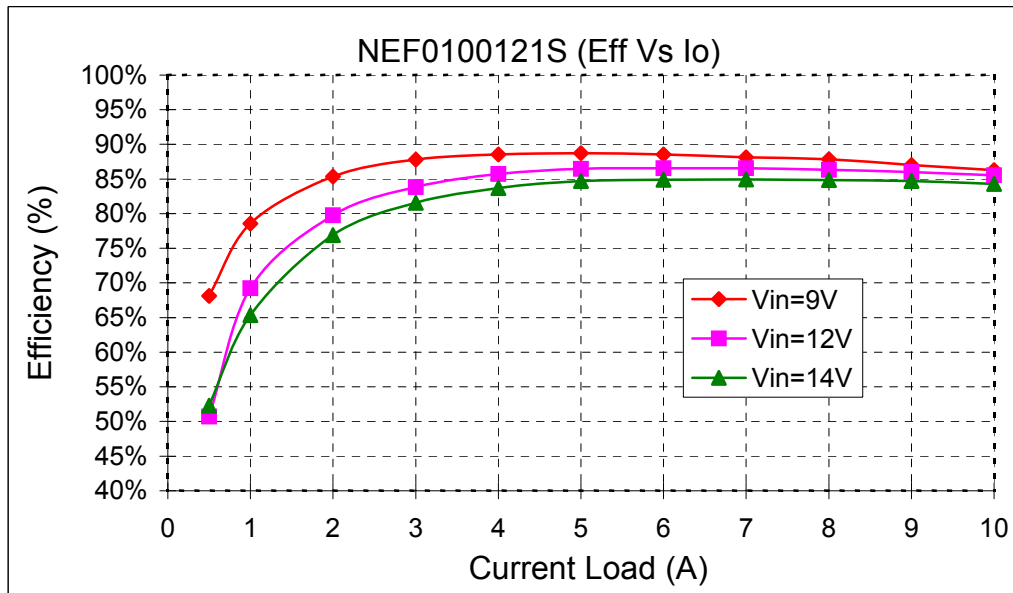
Figure 11. Efficiency Curves for Vout=1.2V (25C)
