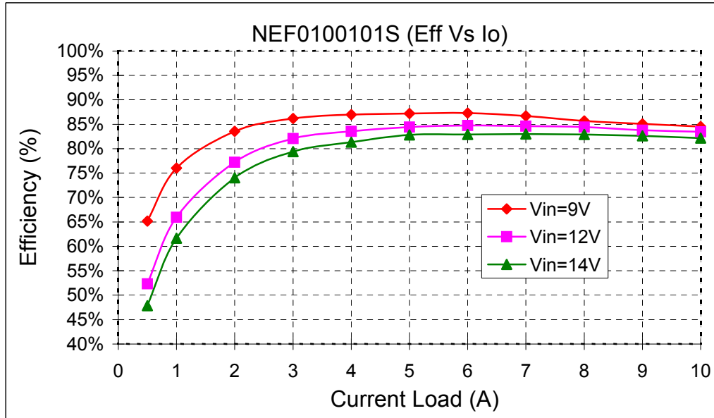
Figure 10. Efficiency Curves for Vout=1.0V (25C)
