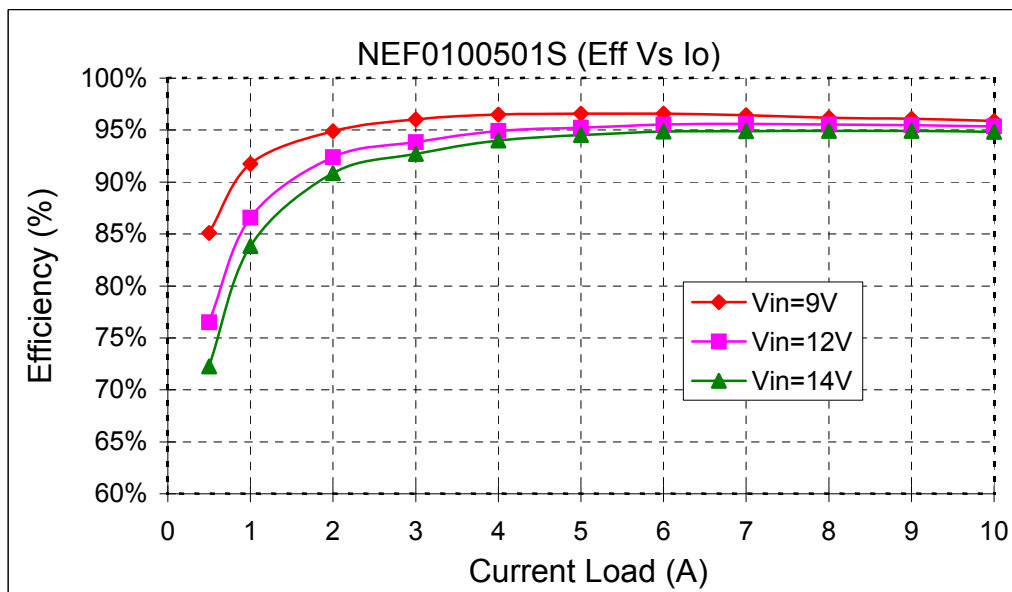
Figure 17. Efficiency Curves for Vout=5.0V (25C)
