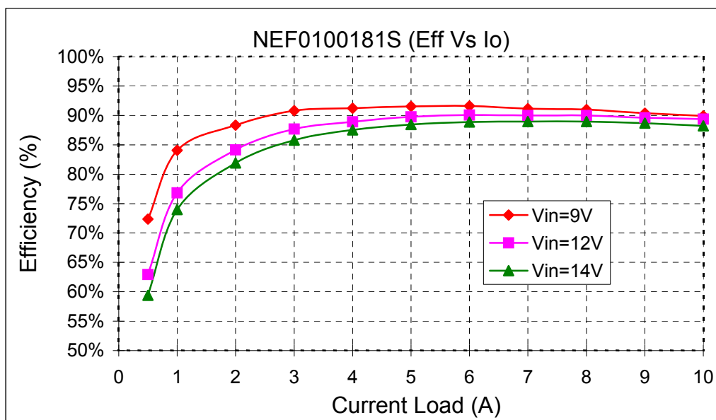
Figure 13. Efficiency Curves for Vout=1.8V (25C)
