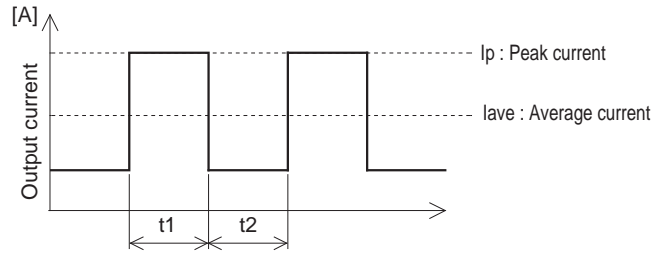
Fig. 7.1 Peak current
