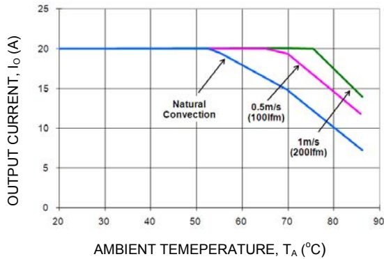
Figure 18. Output Current Derating for the Module with Heatplate; Airflow in the Transverse Direction from V_{out}(-) to V_{out}(+) ; V_{IN} = 24V .
