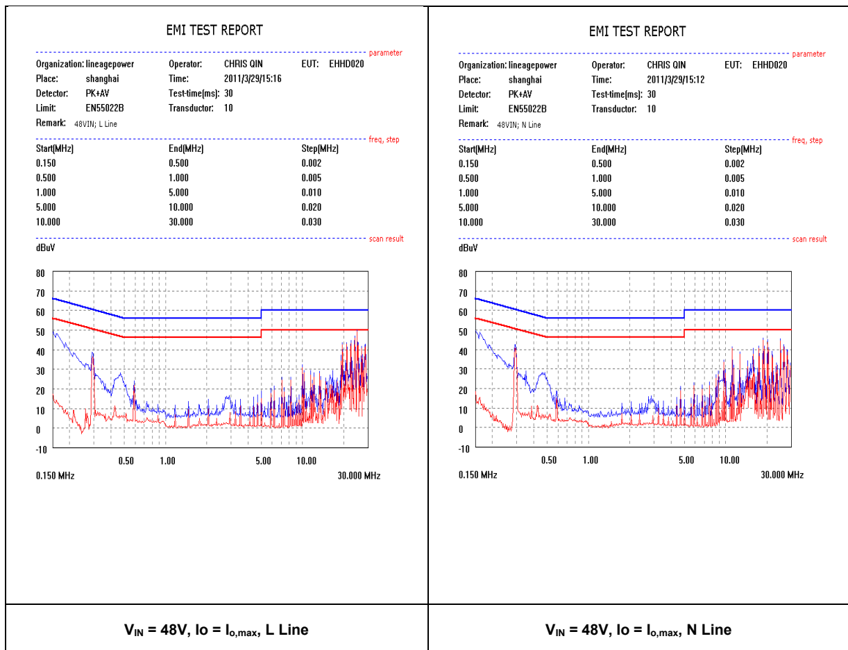
Figure 26. EMC Considerations
