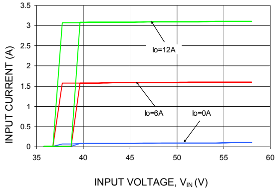
Figure 9. Typical Input Characteristic at Room Temperature.
