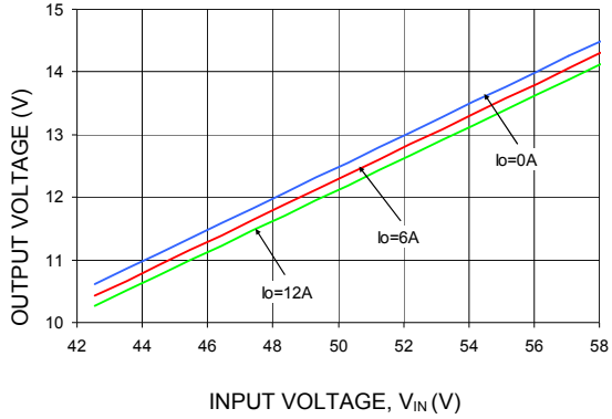
Figure 15. Typical Output voltage Vs. Input voltage Characteristic at Room Temperature.
