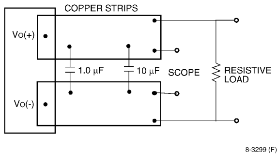
Figure 17. Input Reflected Ripple Current Test Setup.
