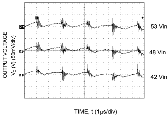
Figure 3. Typical Output Ripple and Noise at Room Temperature and P_o = 200W .
