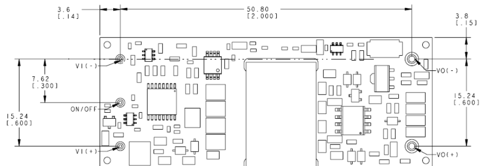
BOTTOM VIEW
