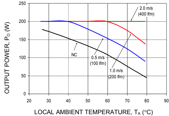
Figure 24. Output Power Derating for the EUE200B1-H ( V_o = 12.0V ) in the Transverse Orientation; Airflow Direction From V_{in}(-) to V_{in}(+) ; V_{in} = 48V .
