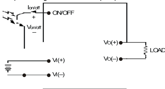
Figure 20. Circuit configuration for using Remote On/Off Implementation.
