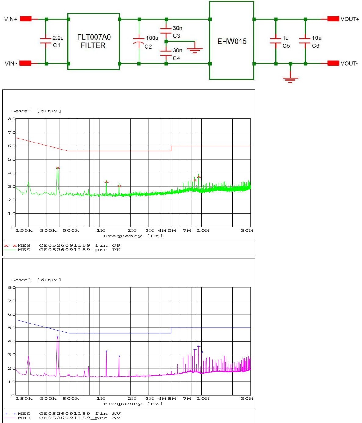
Figure 28. EMC Considerations
