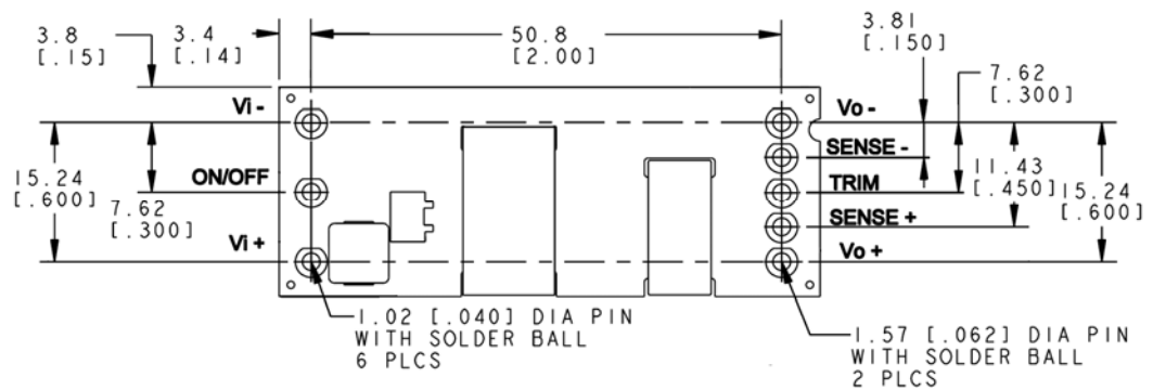
Bottom View
