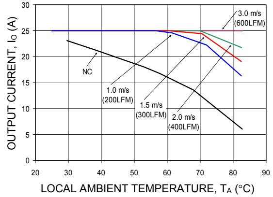
Figure 18. Output Current Derating for the QSW025A0B-H in the Transverse Orientation with baseplate and 0.5-inch high heatsink; Airflow Direction from Vin(+) to Vin(-); Vin = 48V.
