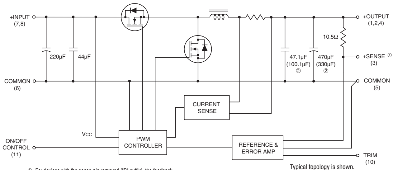
Figure 1. Simplified Schematic
